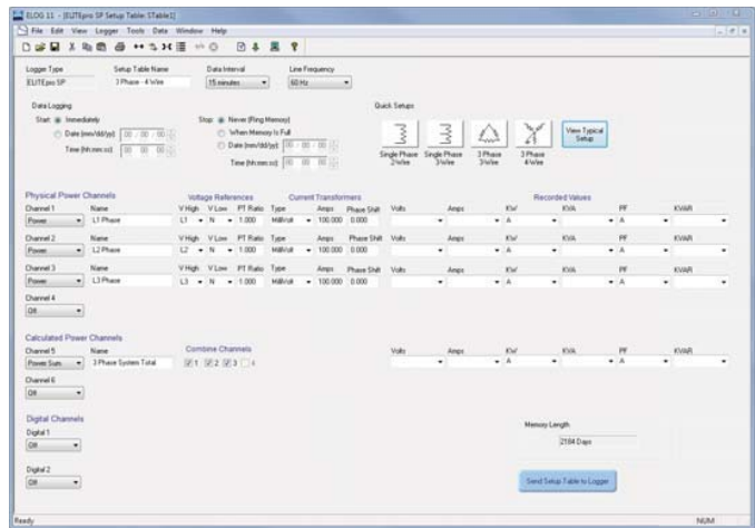
Flexible Options: Configure the ELITEpro SP for a variety of measurement projects with a few mouse clicks.
