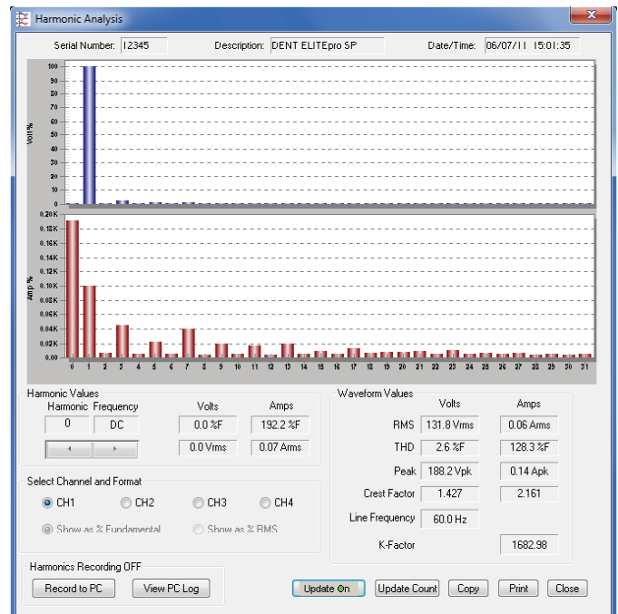
Perform Harmonic Analysis on a connected load. View harmonic and waveform values in real time. Line frequency is also displayed as a real-time value.
